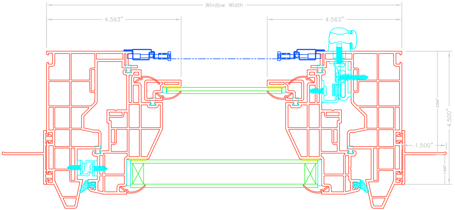
Section B-B
