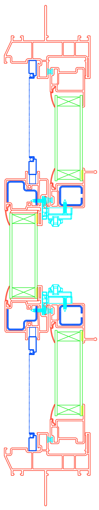
Section B-B
