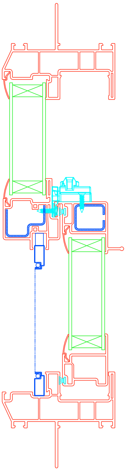
Section B-B
